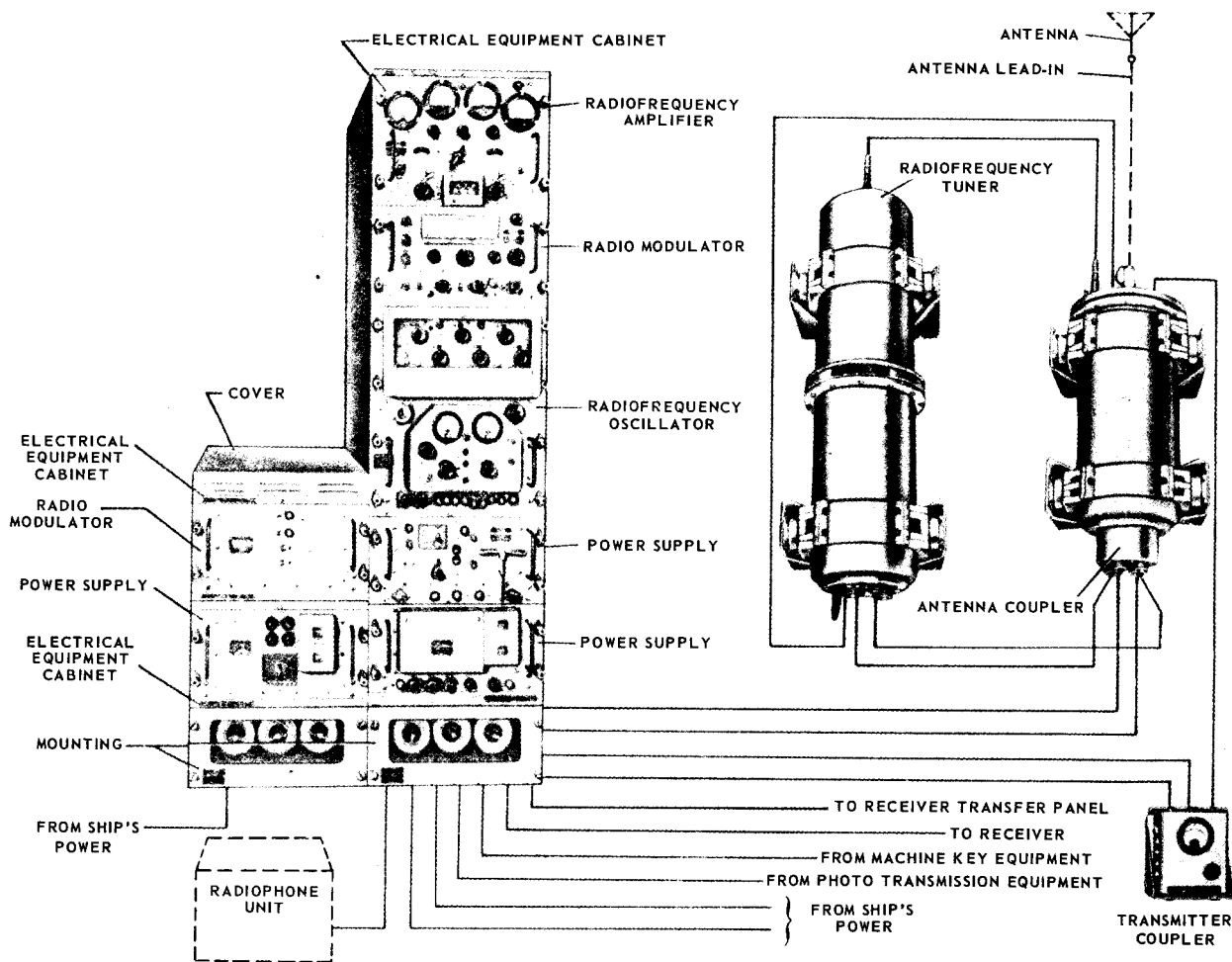
1. 144 Figure 9-11. —Radio transmitter AN/SRT-15.
