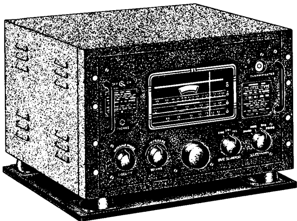
Figure 9-30.—Model RBO entertainment receiver.
