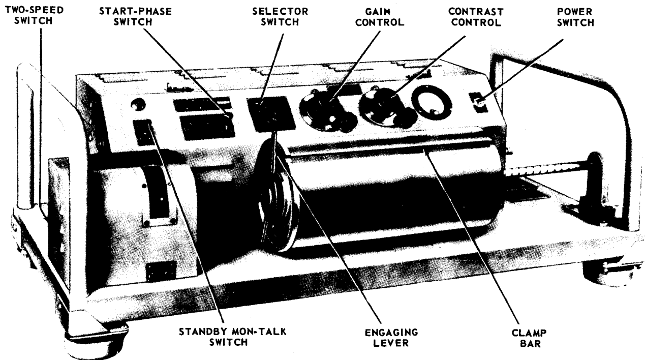
Figure 9-34. – Facsimile transceiver TT-41B/TXC-1B.
