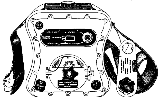
Figure 9-45. — Emergency lifeboat transmitter AN/CRT-3.
