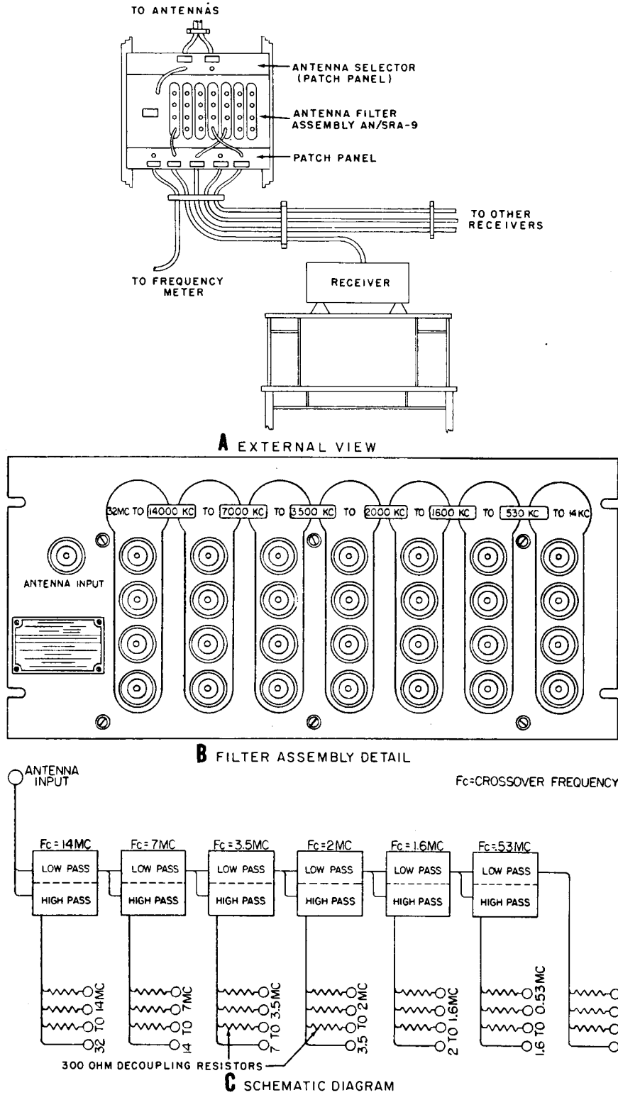
Figure 9-40. —Receiving antenna distribution system, using antenna filter assembly. 1.51:115
