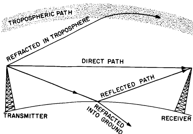
Figure 8-8. — Possible routes for groundwaves. 31.12
