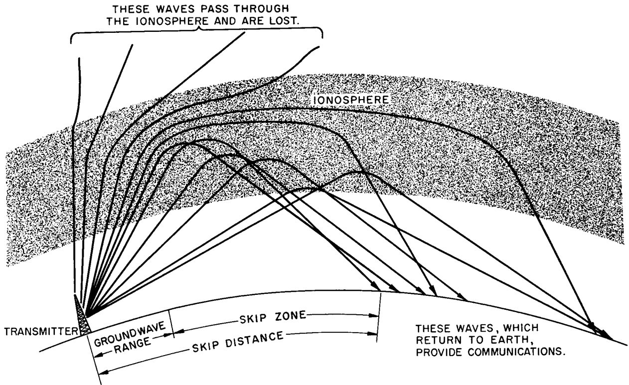
Figure 8-12. —Skywave transmission paths.
