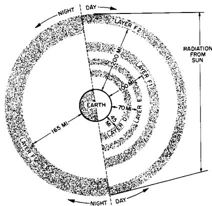
Figure 8-11. —Ionosphere layers 31. 15
