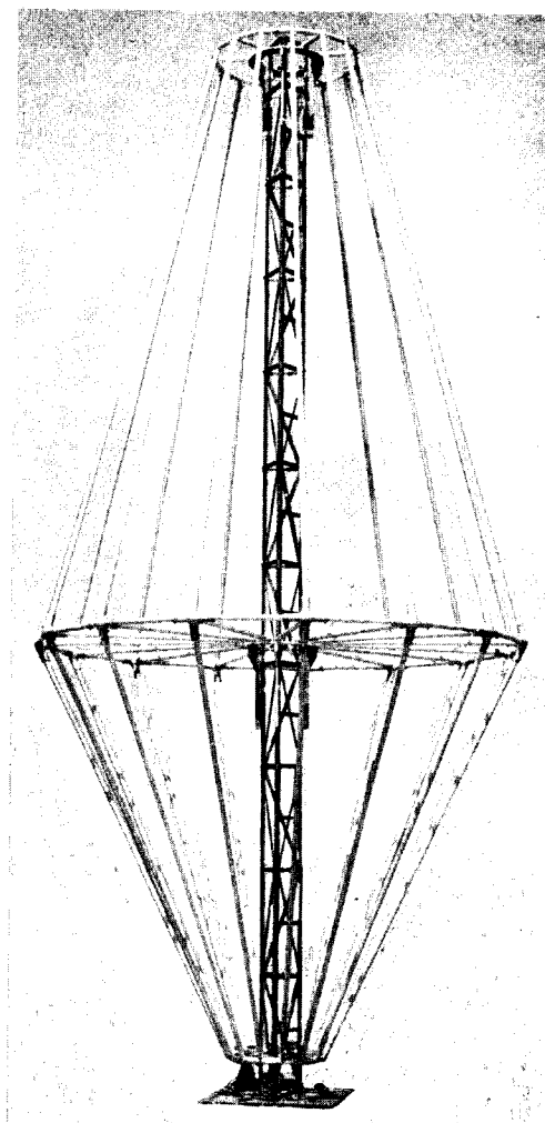
Figure 8-26. —Conical monopole antenna.
