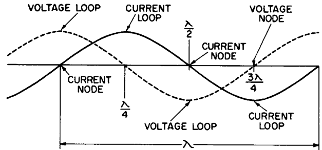
Figure 8-21. — Standing waves along full-wave antenna. 76.14
