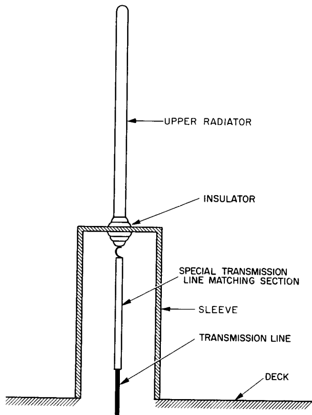
Figure 8-25. —Sleeve antenna (shipboard).
