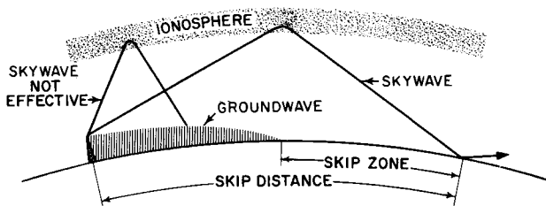
Figure 8-13. —Relation of skip zone and groundwave.
